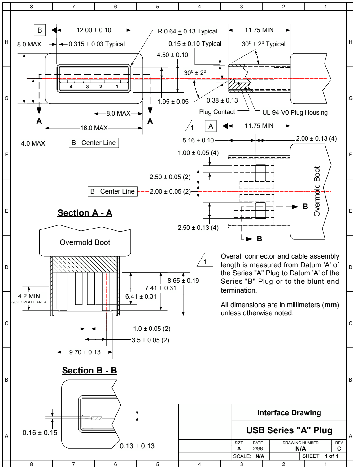
USB Series "A" Plug Interface Drawing
