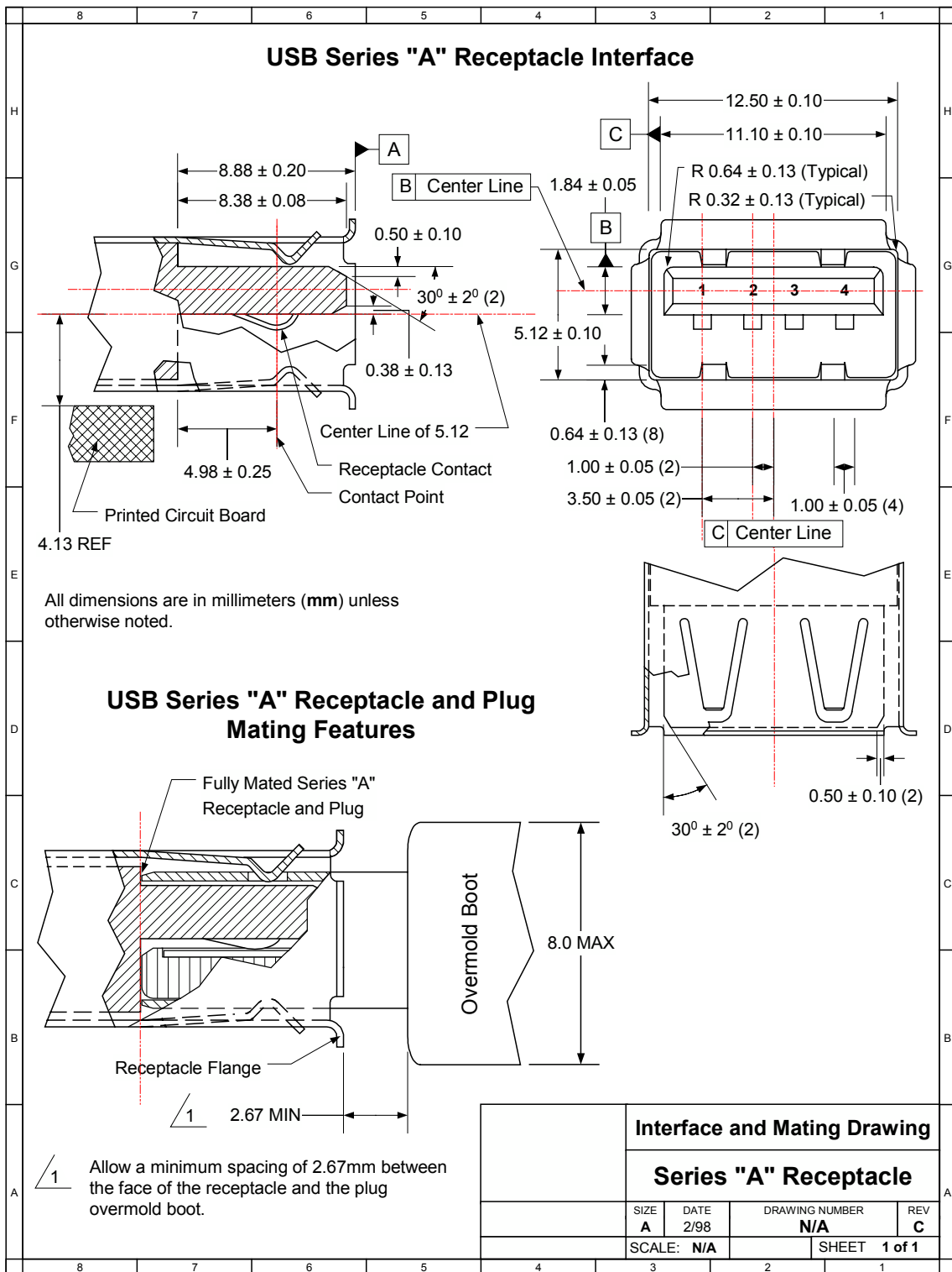
USB Series "A" Receptacle Interface and Mating Drawing
